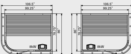
Space Vision 250, front entrance. (External roof height 79.92")
