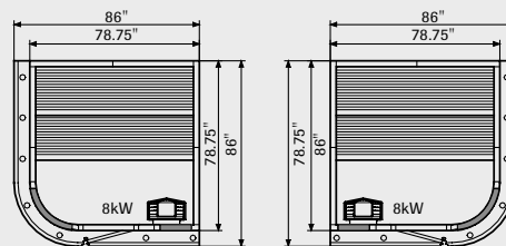
Midi Vision (External roof height 79.92")
