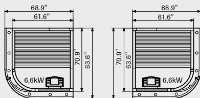
Space Vision 150, corner entrance. (External roof height 79.92")
